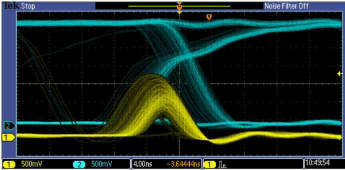
Digital phosphor technology enables a 5,000 wfm/s waveform capture rate and real-time intensity grading on the MSO/DPO2000 Series.
